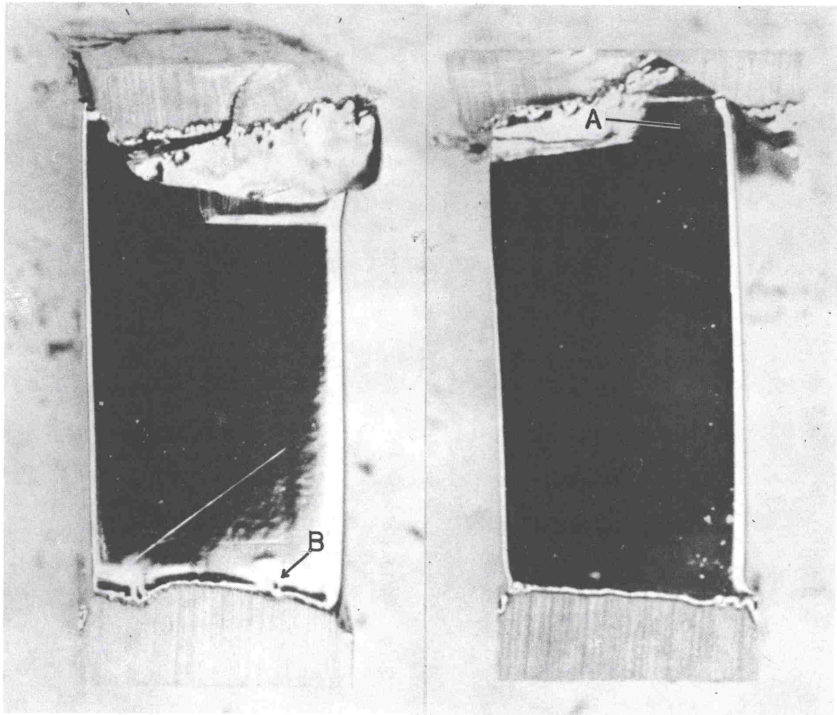
Fig. 14 - Macrophotograph Showing \{11\bar{2}0\} and \{\bar{1}010\} Lateral Surfaces of Crystal SR-11-1 After c-axis Compression Under Hydrostatic Pressure in the Range 156-164 ksi.
